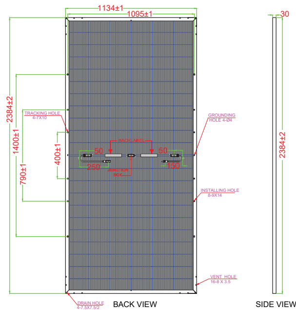
Fig 4: Mechanical Drawing of PV module HYPERSOL VSM DH.66.AAA.05
