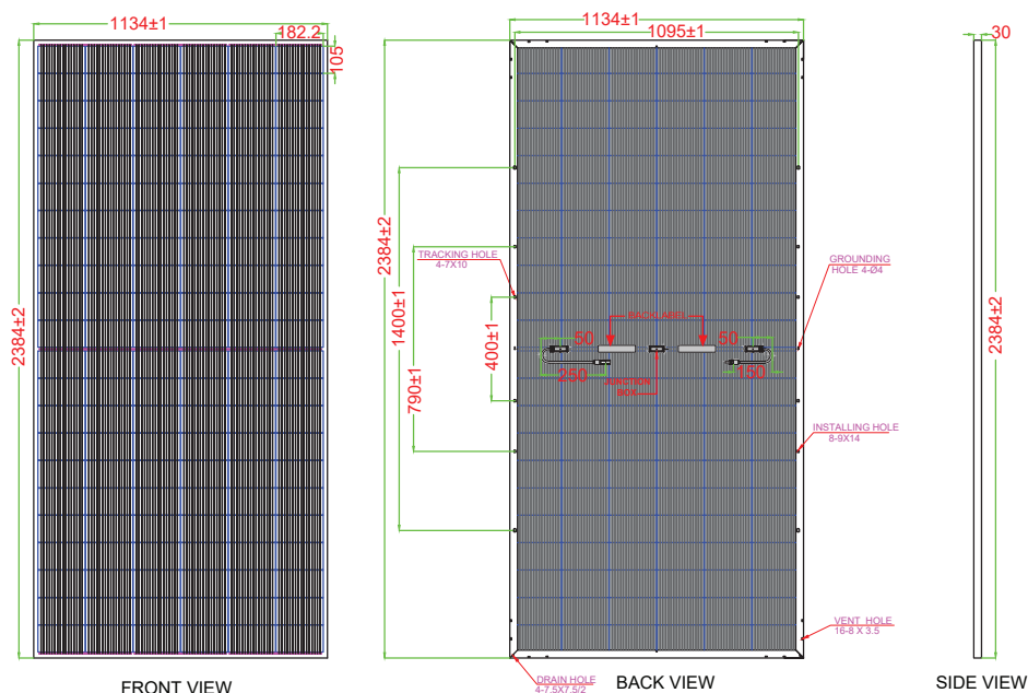
Fig 3: FRONT VIEW & BACK VIEW
