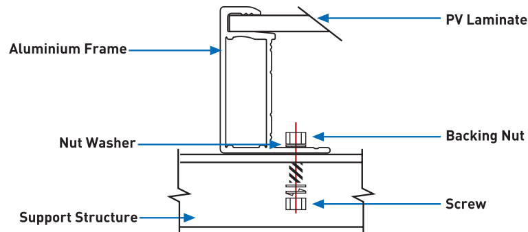
Fig 5: Modules Installed with Screw Fitting Method
