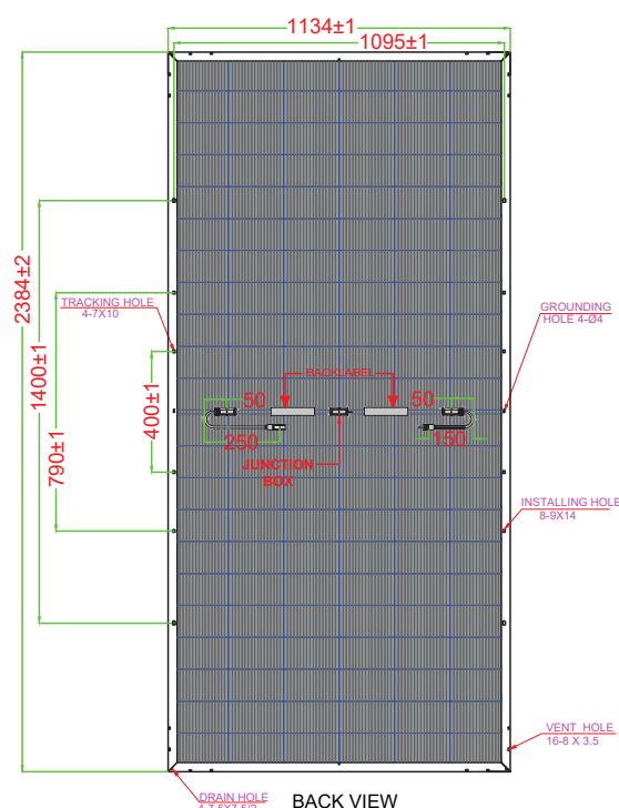
Fig 2: BACK VIEW GLASS TO GLASS BIFACIAL MODULE
