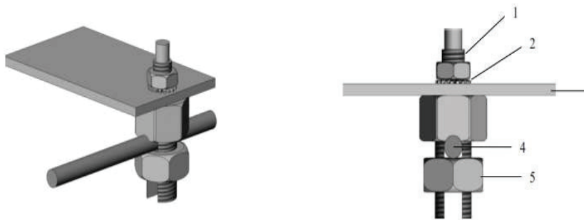
Fig 9 Grounding bolt # 2058729-1
