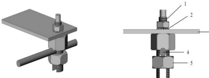
Fig 9: Grounding bolt # 2058729-1
