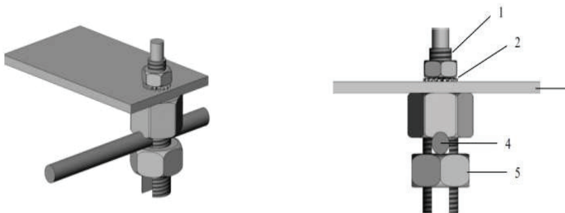
Fig 10: Grounding bolt # 2058729-1
