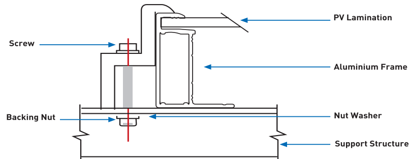
Fig 8: PV modules installed using fringe clamping method
