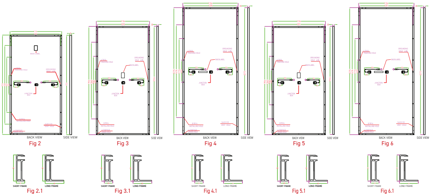
Fig 2: Mechanical Drawing of PV module SOMERA VSMH.54.AAA.05, PREXOS VSMH.60.AAA.05 and SOMERA VSMH.72.AAA.05
