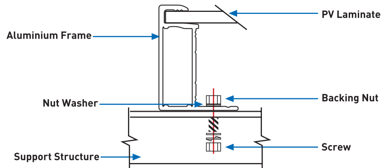
Fig 7: Modules Installed with Screw Fitting Method
