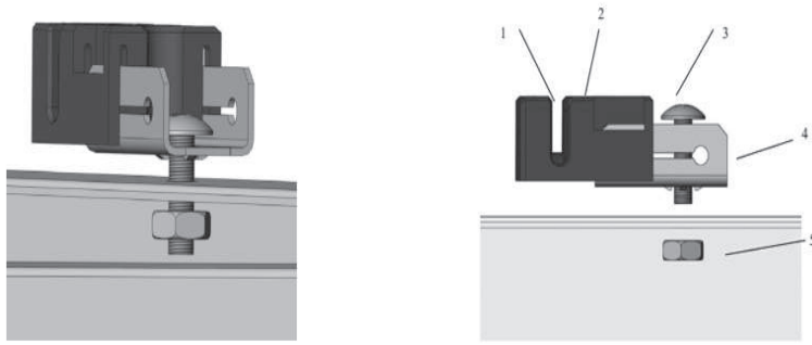
Fig 11: Grounding bolt # 1954381-2
